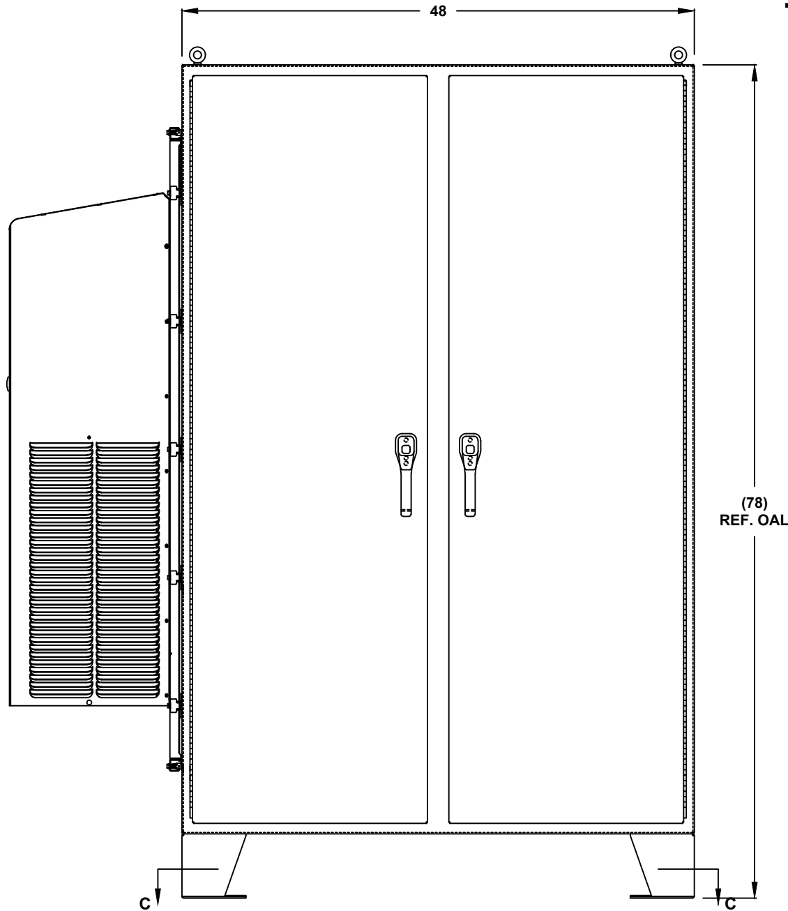
FRONT VIEW
