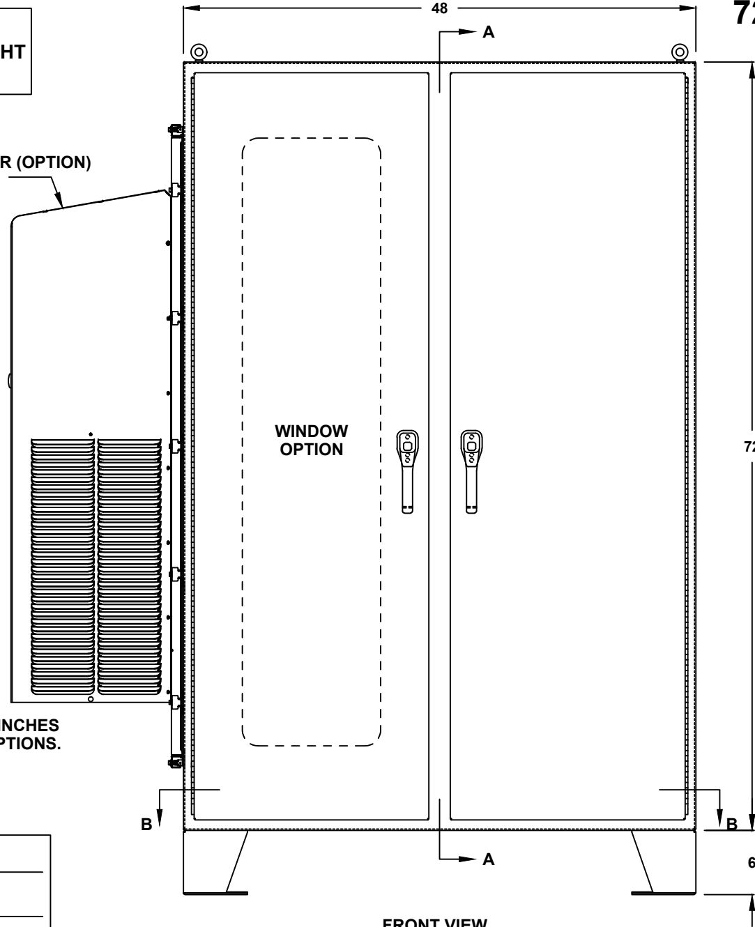
FRONT VIEW
